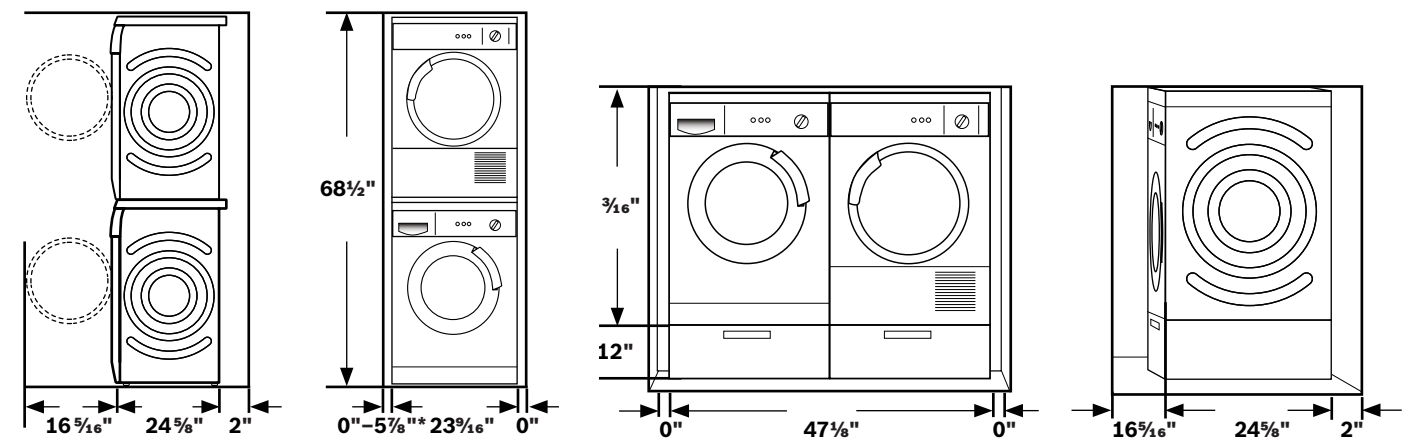
Closet installation with WTE863100US
