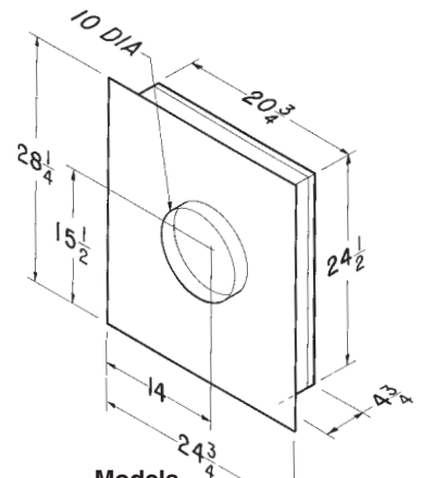
Models 331H & 332H Exterior Blowers
