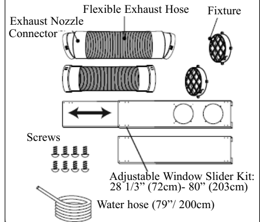
Fig. 1 INSTALLATION ACCESSORIES
