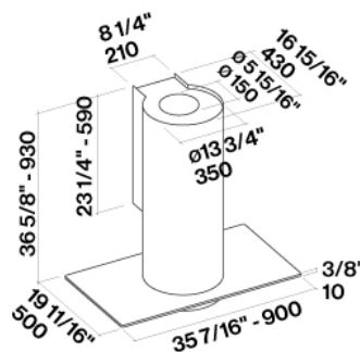
Hood with optional glass (FDPGL36W0TG)
