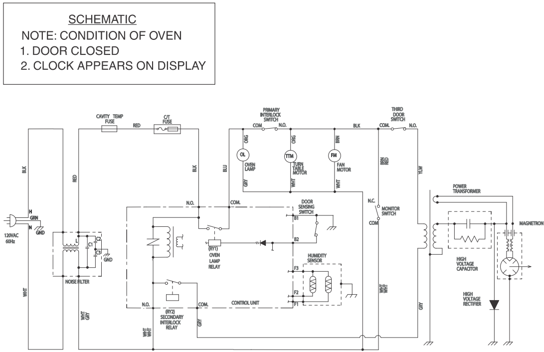
Figure O-1 Oven Schematic - Off Condition
