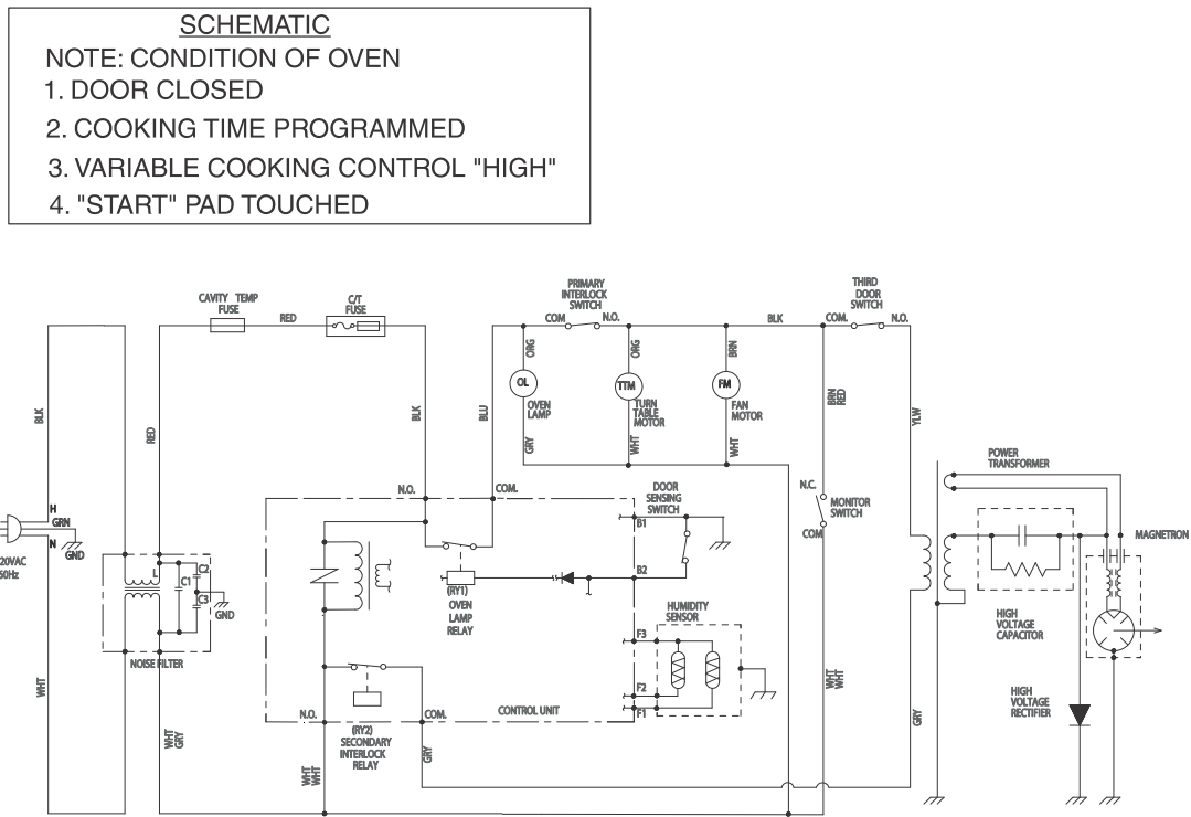
Figure O-2 Oven Schematic - Cooking Condition
