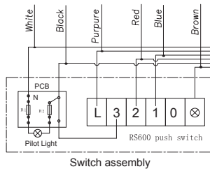
Switch assembly
