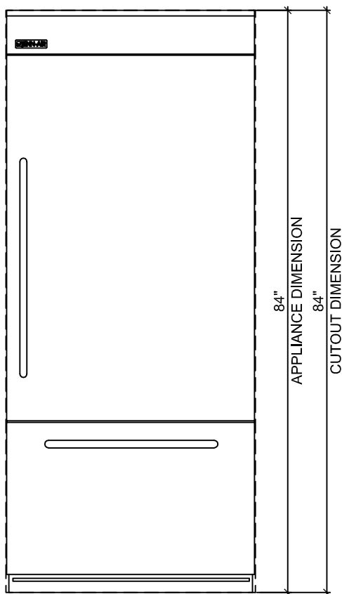
2 FRONT ELEVATION
