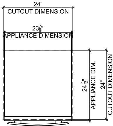
1 PLAN
