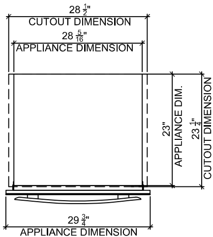
1 PLAN
