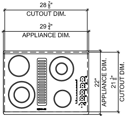
1 PLAN
