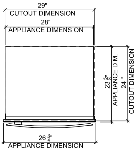
1 PLAN
