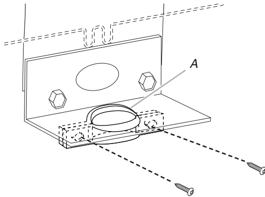
A. UL listed strain relief
