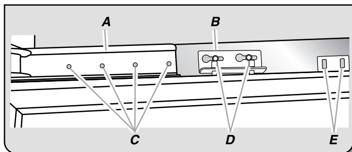
A. Top hinge B. Mounting bracket C. Holes for screws
