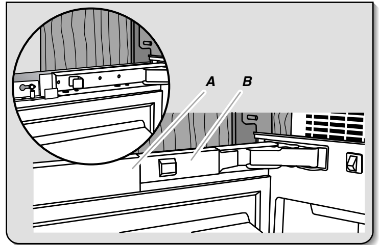
A. Door adjustment pin cover B. Top hinge cover
