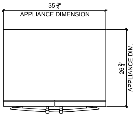
1 PLAN
