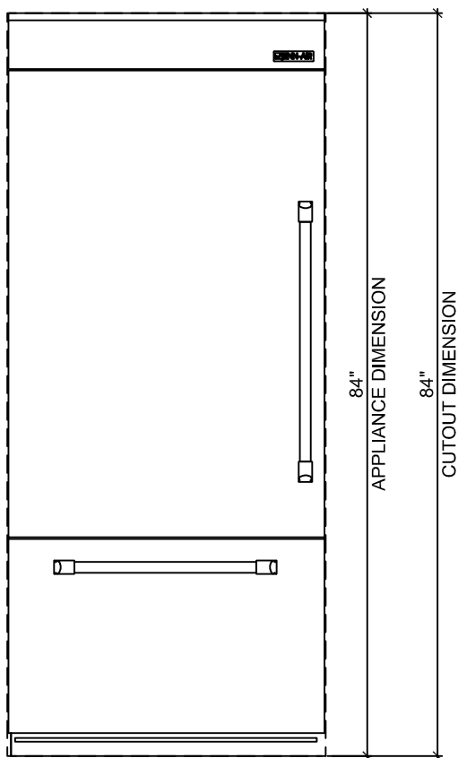
2 FRONT ELEVATION
