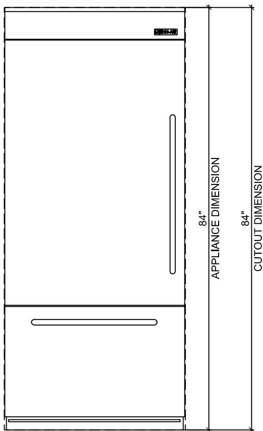
2 FRONT ELEVATION
