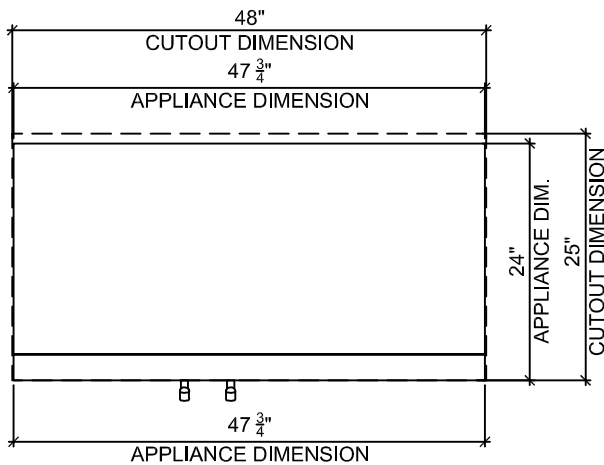
1 PLAN
