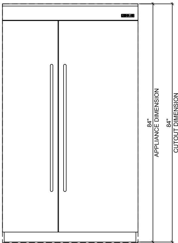
2 FRONT ELEVATION
