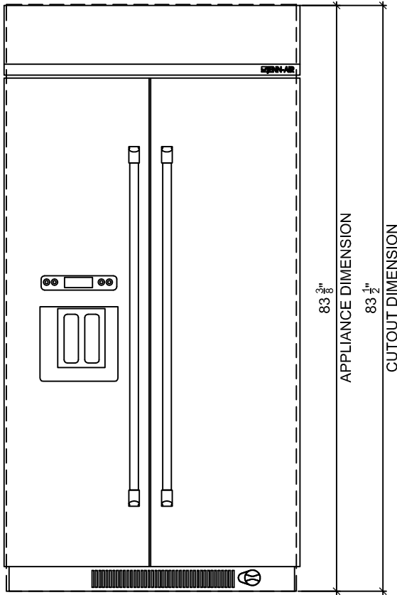
2 FRONT ELEVATION
