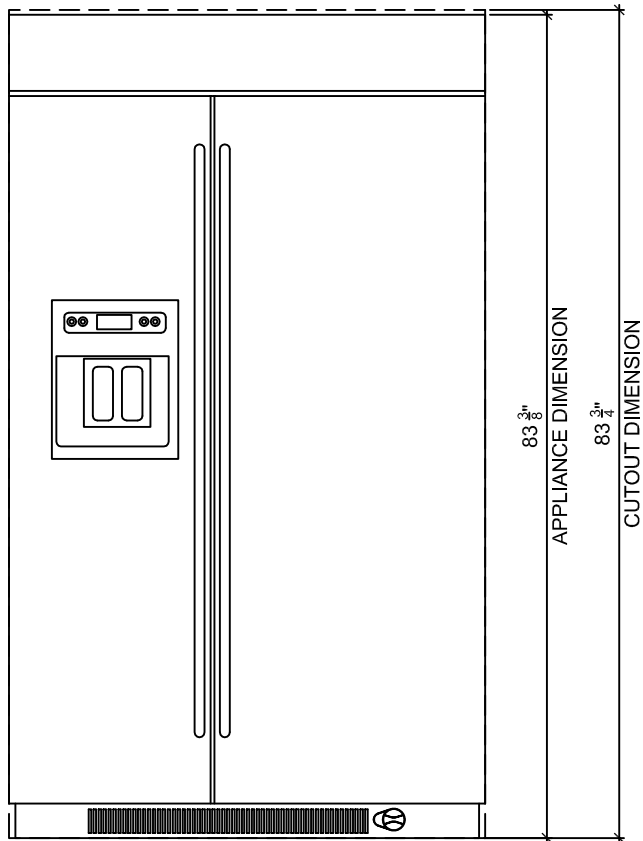
2 FRONT ELEVATION
