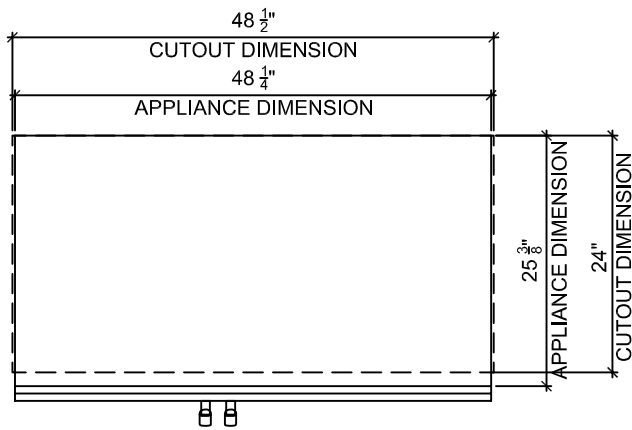
1 PLAN
