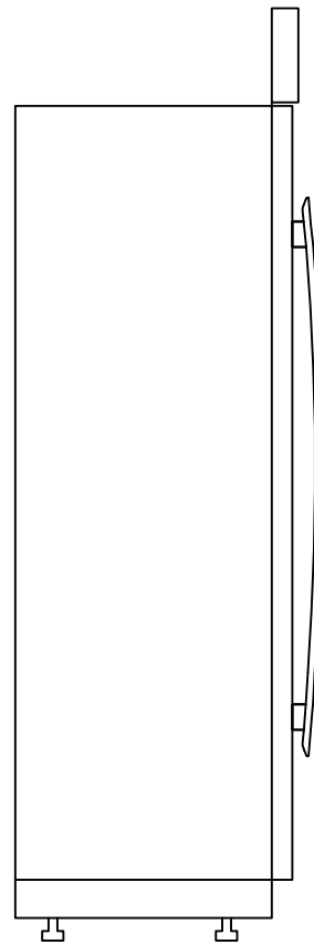
3 SIDE ELEVATION
