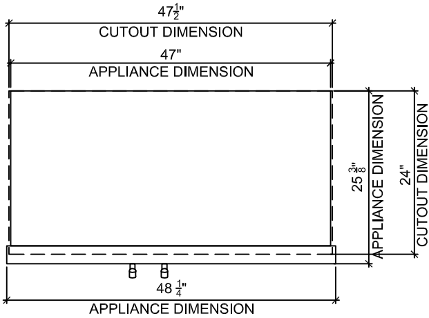
1 PLAN
