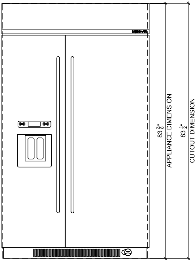
2 FRONT ELEVATION
