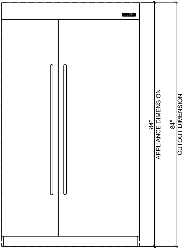
2 FRONT ELEVATION
