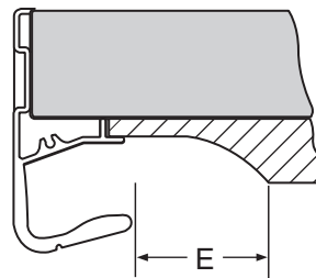
Handle Clearance for Raised Panel
