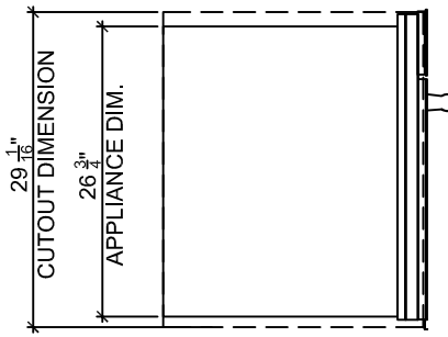
3 SIDE ELEVATION
