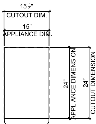
1 PLAN
