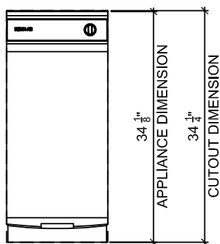
2 FRONT ELEVATION
