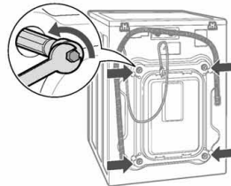
Unpacking and removing shipping bolts
