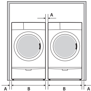
Recessed area
