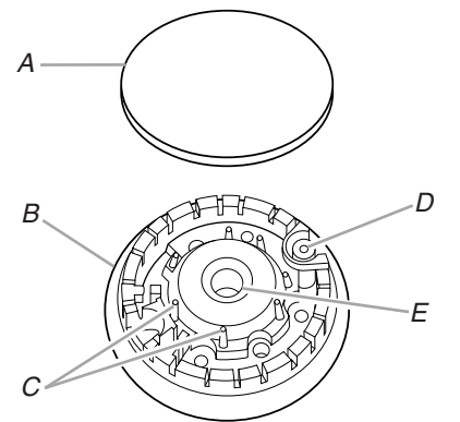
A. Burner cap C. Alignment pins B. Burner base D. Igniter E. Gas tube opening
