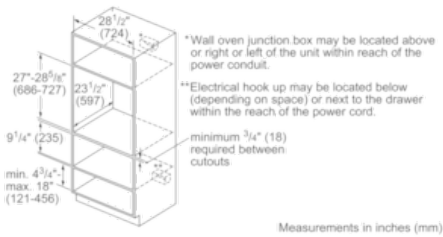
Standard Installation 30" Single Oven over Storage or Warming Drawer
