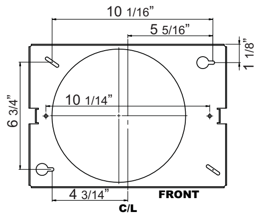
TOP SUPPORT FRAME (top view)
