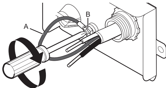
A. Ground wire B. Ground screw
