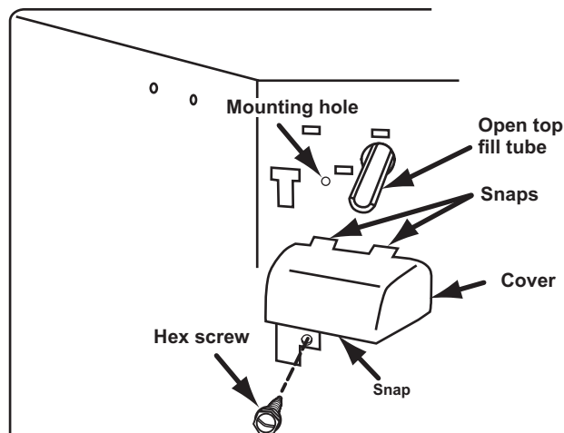
Removing wiring cover with open-top fill tube
