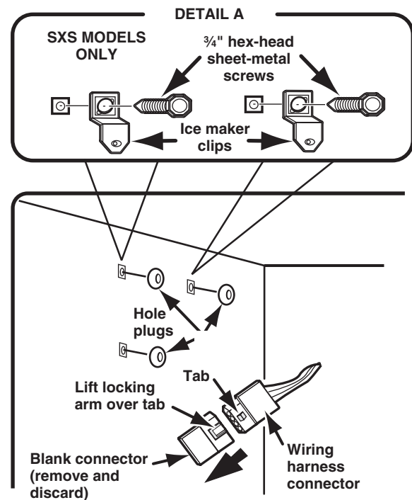
Installing the ice maker clips
