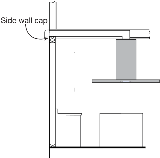
TOP VENTING WALL EXHAUST
