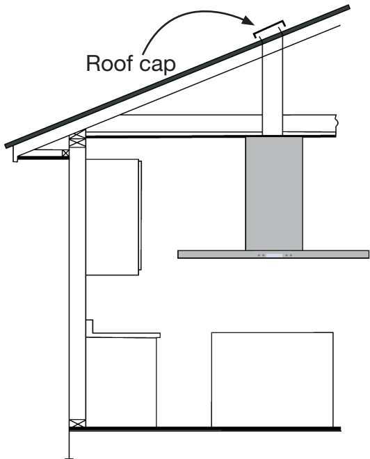
TOP VENTING ROOF EXHAUST
