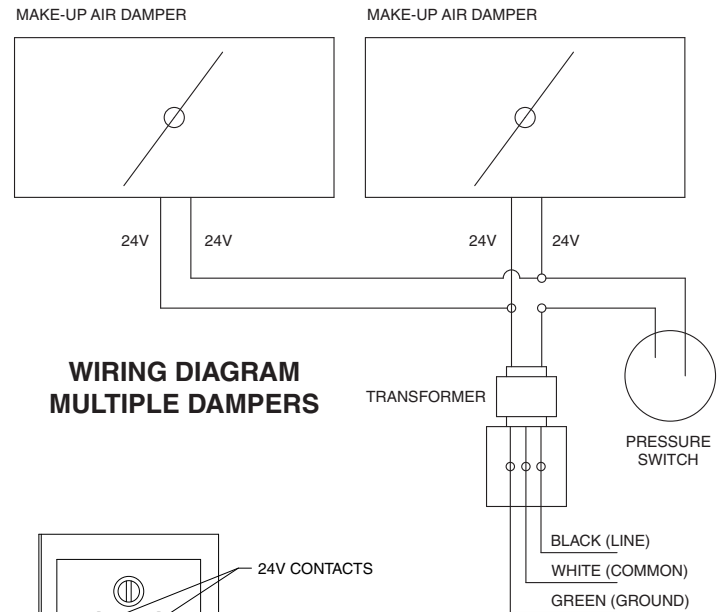
TRANSFORMER WIRING
