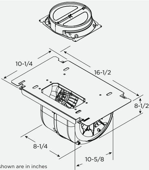
Dimensions shown are in inches
