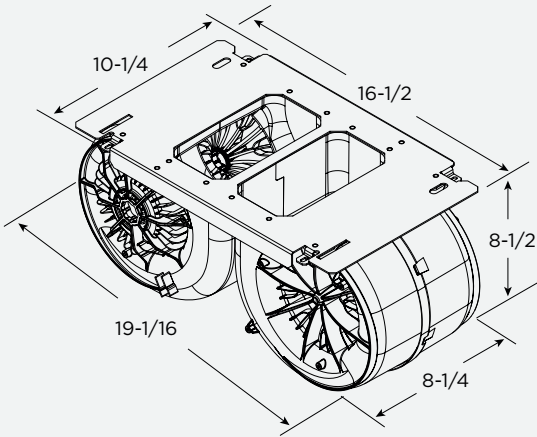
Dimensions shown are in inches
