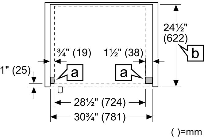
Top view right swing door
