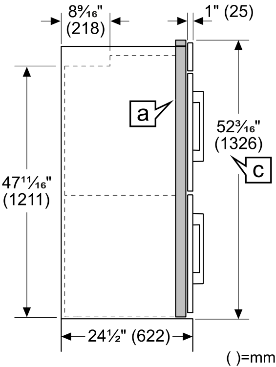
Side view (representative)
