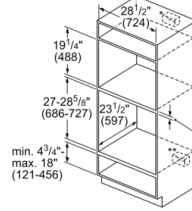
Standard installation 30" speed oven or microwave above a single oven***
