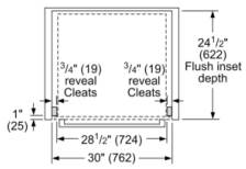
Flush installation Top view
