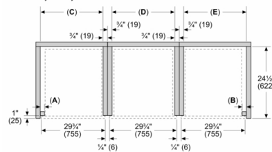
Flush side-by-side-by-side installation
