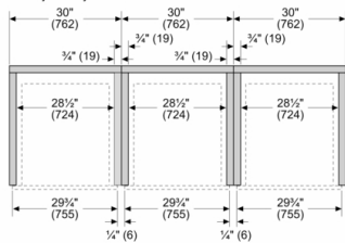
Standard side-by-side installation
