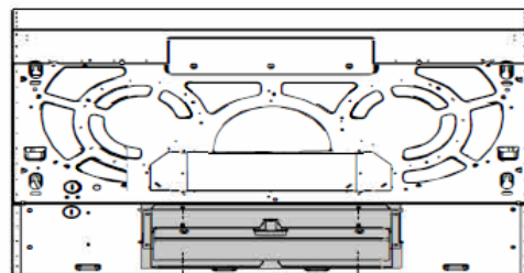
3 1/4"x14" DAMPER
