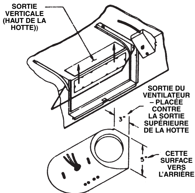
FIGURE 4 – SORTIE VERTICALE
