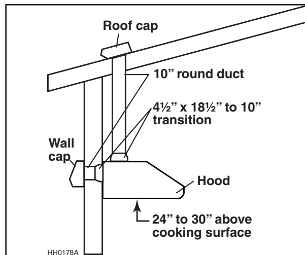
DOUBLE INTERNAL BLOWERS TYPICAL DUCTWORK
