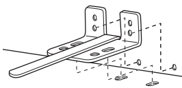
Minimum Acceptable #2 – Wood Floor
