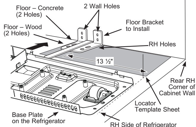
Figure 1 – Installation Overview
