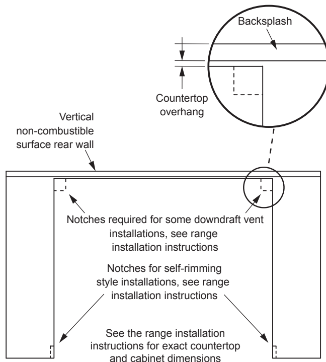
Range Cabinet/Countertop Cutout - Top View
