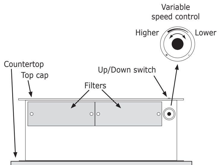
Parts the of Downdraft Vent - Shown Raised
