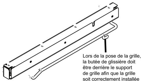
Figure 9 : Installation des grilles Luxury Glide™
