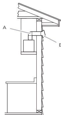
Wall venting
