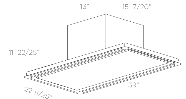
FALSE CEILING CUT: 21 13/20" x 38 1/2"
