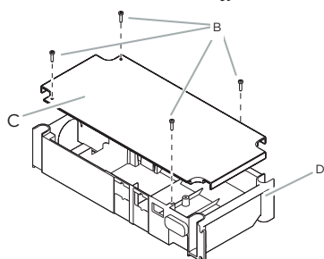
A. Bracket B. Terminal box screws C. Terminal box cover D. Terminal box
