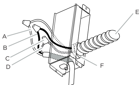
A. White wires B. Black wires C. UL listed wire connectors D. Green (or bare) and yellow-green ground wire E. Home power supply cable F. UL listed or CSA approved 1/2" strain relief
