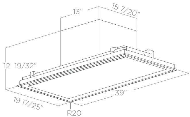
FALSE CEILING CUT: 18 57/64 X 38 37/64
