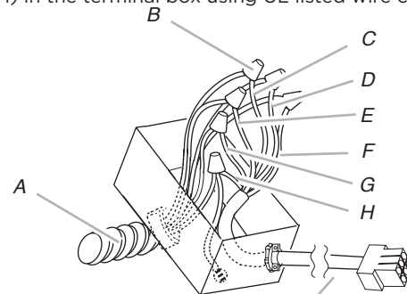
A. Strain relief B. UL listed wire connectors C. Black wires D. White wires E. Red wires F. Blue wires G. Gray wires H. Green (or yellow/ green) and green / yellow wires I. Motor electrical plug cable
