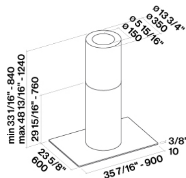
Hood with optional glass (FDPGL36I0TG)
