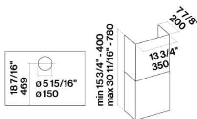
Rear view and optional chimney
